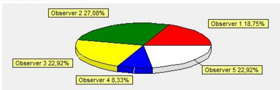
Comparison of shower meteors
