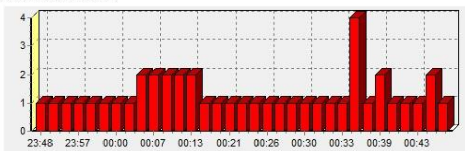
Minute frequency of meteors
